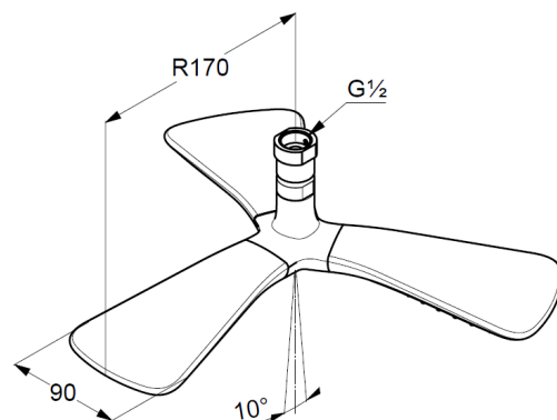
Dimensional drawing
